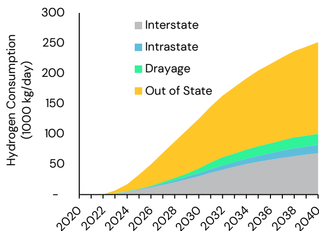
Figure 14 - Estimated Class 8 Hydrogen Consumption in LA County
