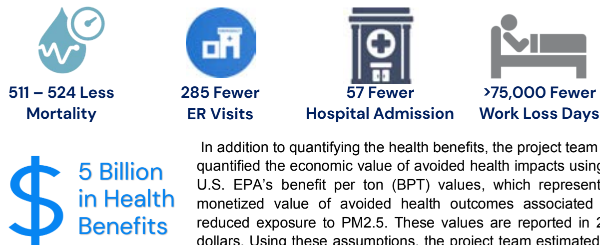
Figure 12. Cumulative (2024-2040) health benefits associated with emissions reductions from Class 8 trucks in LA County
