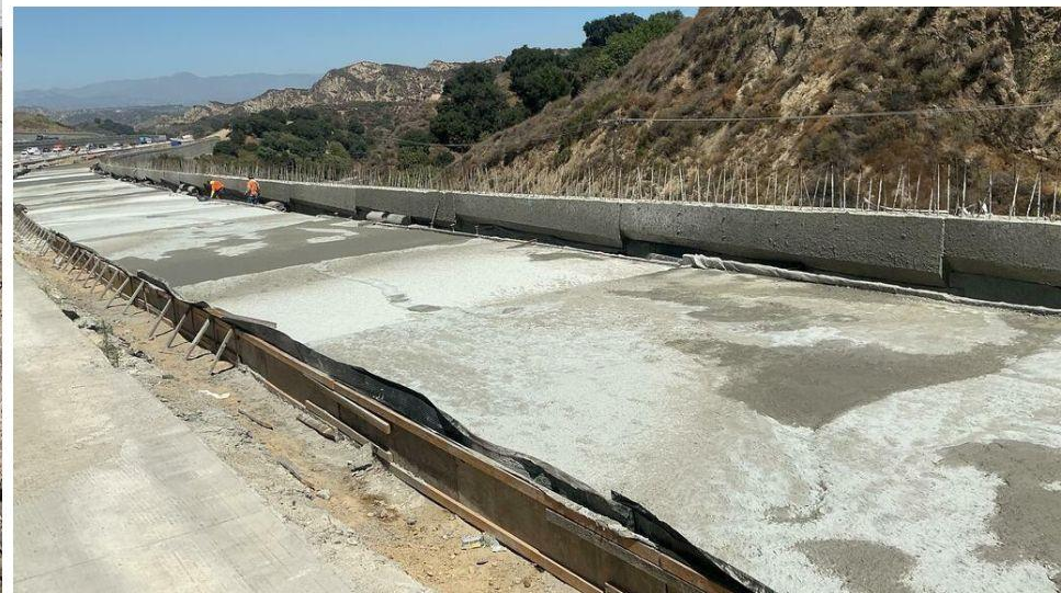
Southbound retaining wall concrete placement and paving – August 2025
