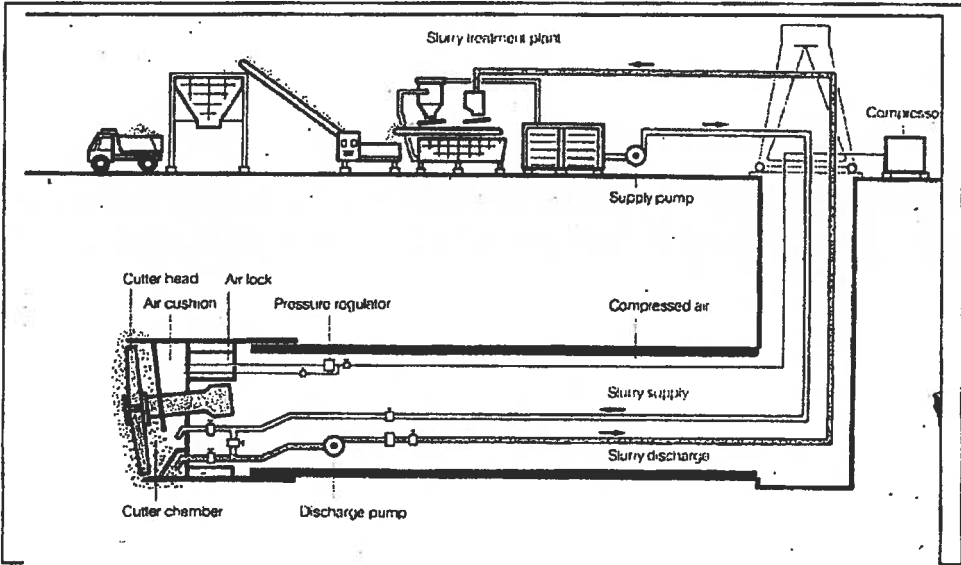
Figure C-2 Slurry Material Conveyance
