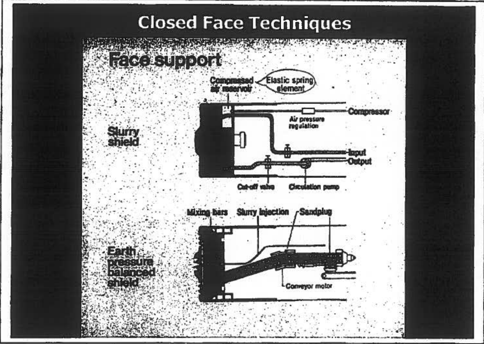
Figure C-1 Slurry and EPB TBM
