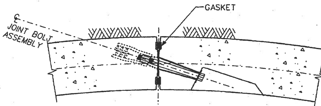
Figure 1 Double Gasket Liner
