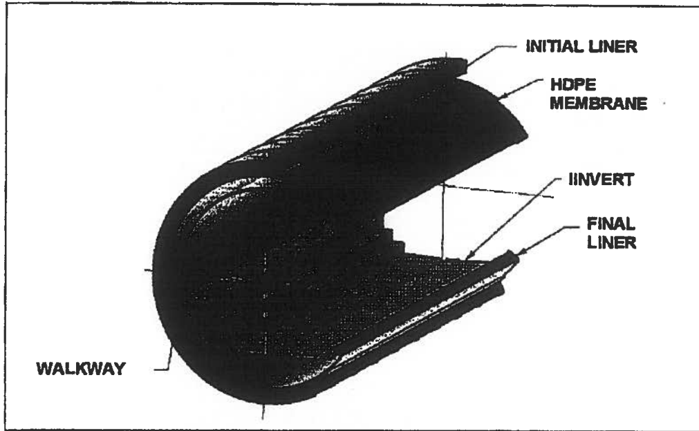
Figure C-5 Tunnel Liners and Membrane Orientation
