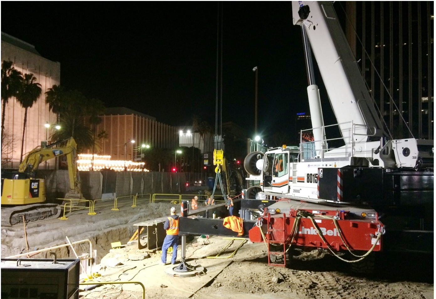
Wilshire/Fairfax Station Deck Beam and Decking Installation Activities
