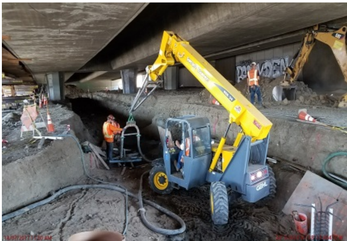
Pedestrian overcrossing piles.
