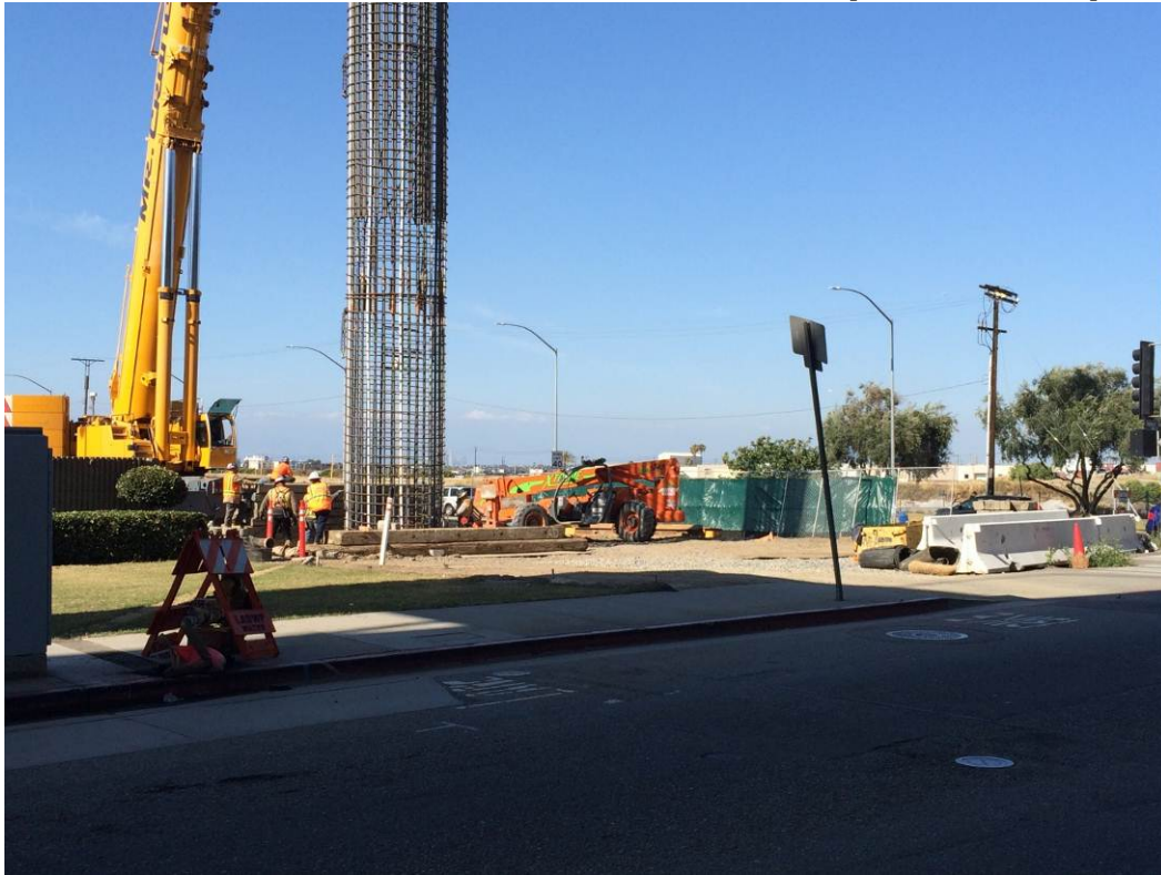
Green Line Underpass Bent 5 Column Rebar Cage Placement.
