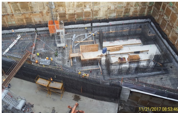
North concourse rebar and electrical installation
