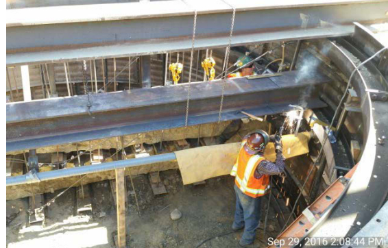
Excavation and utility hanging at Tie-back Removal Pit
