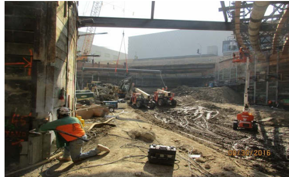
Tie-back related work at 2 nd /Hope Station
