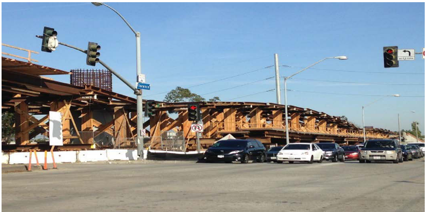
(AG-5) I-405 Bridge – Bridge superstructure falsework erection 90% complete. Crews commenced rolling soffit construction in frame 1.
