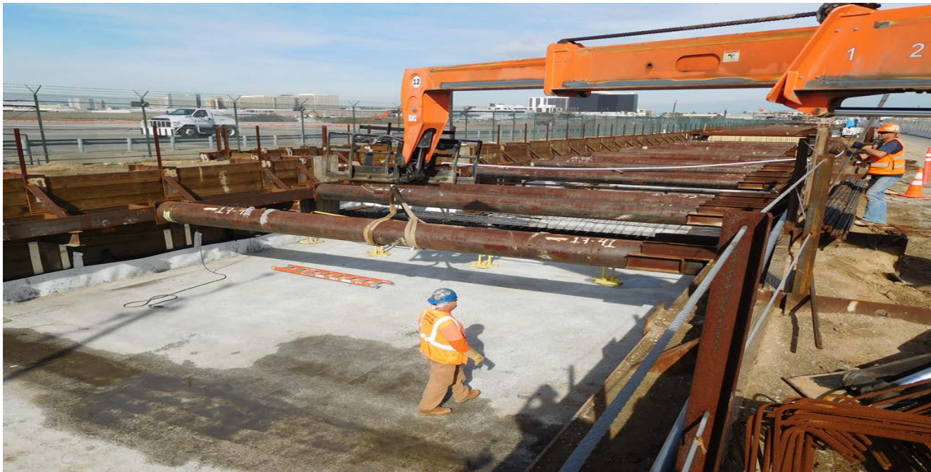
UG#1 Tier 1 SOE strut removals ongoing.
