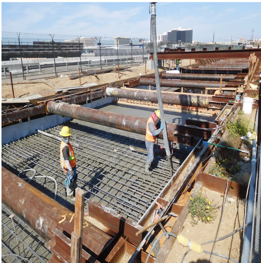
UG#1 - Concrete placement for cut-and-cover tunnel segment.
