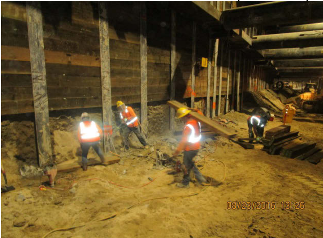
UG#4 – Excavation and lagging along west wall.
