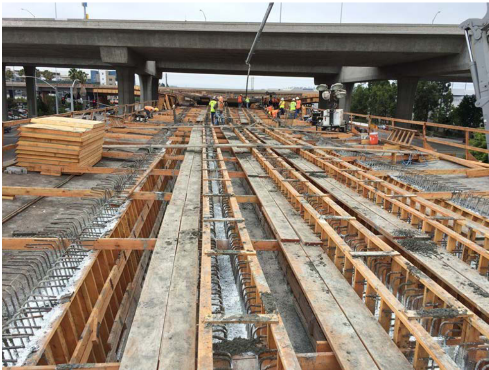
GREENLINE UNDERPASS – Frame 2 pour looking down at station.
