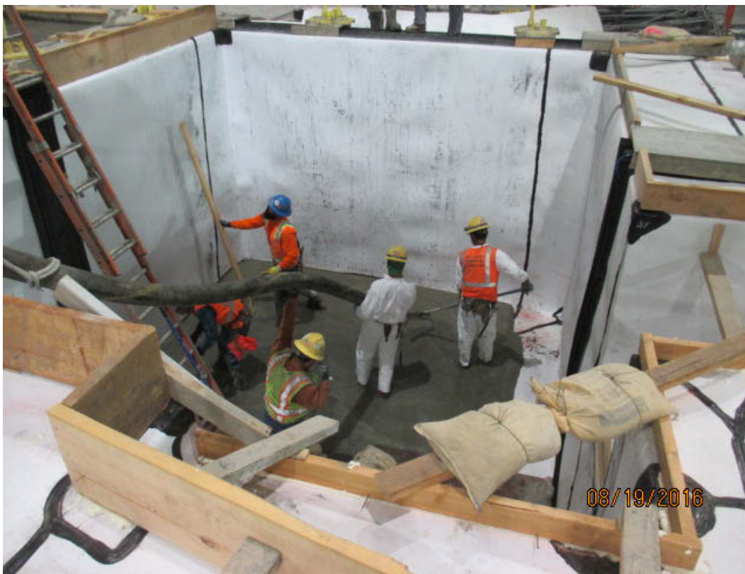
LEIMERT PARK STATION – Placement of protection slab at sump pit.
