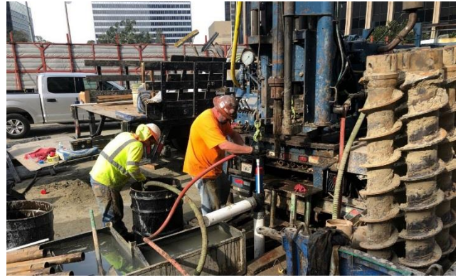
Annular Space Grouting between Inclinator and Conductor Casing for Pile Installation
