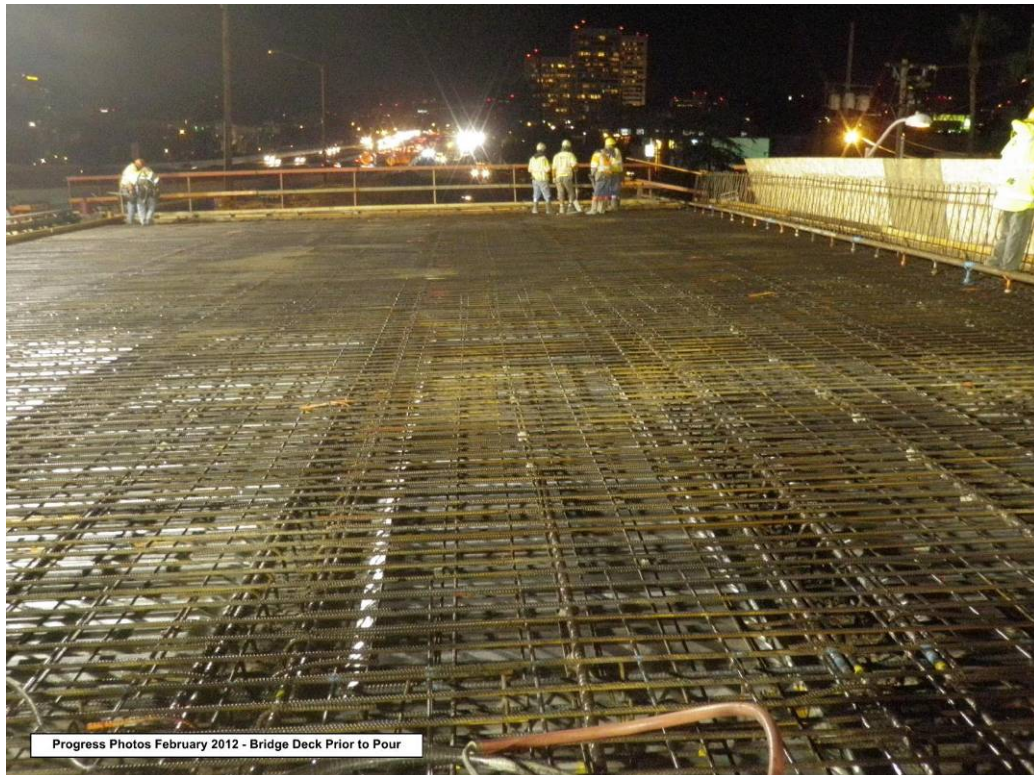
Bridge deck prior to pour.
