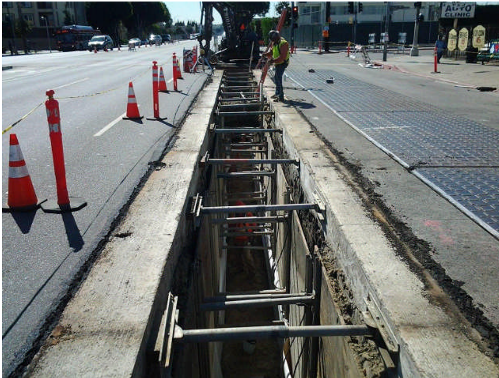
Excavation and shoring along Crenshaw Boulevard.
