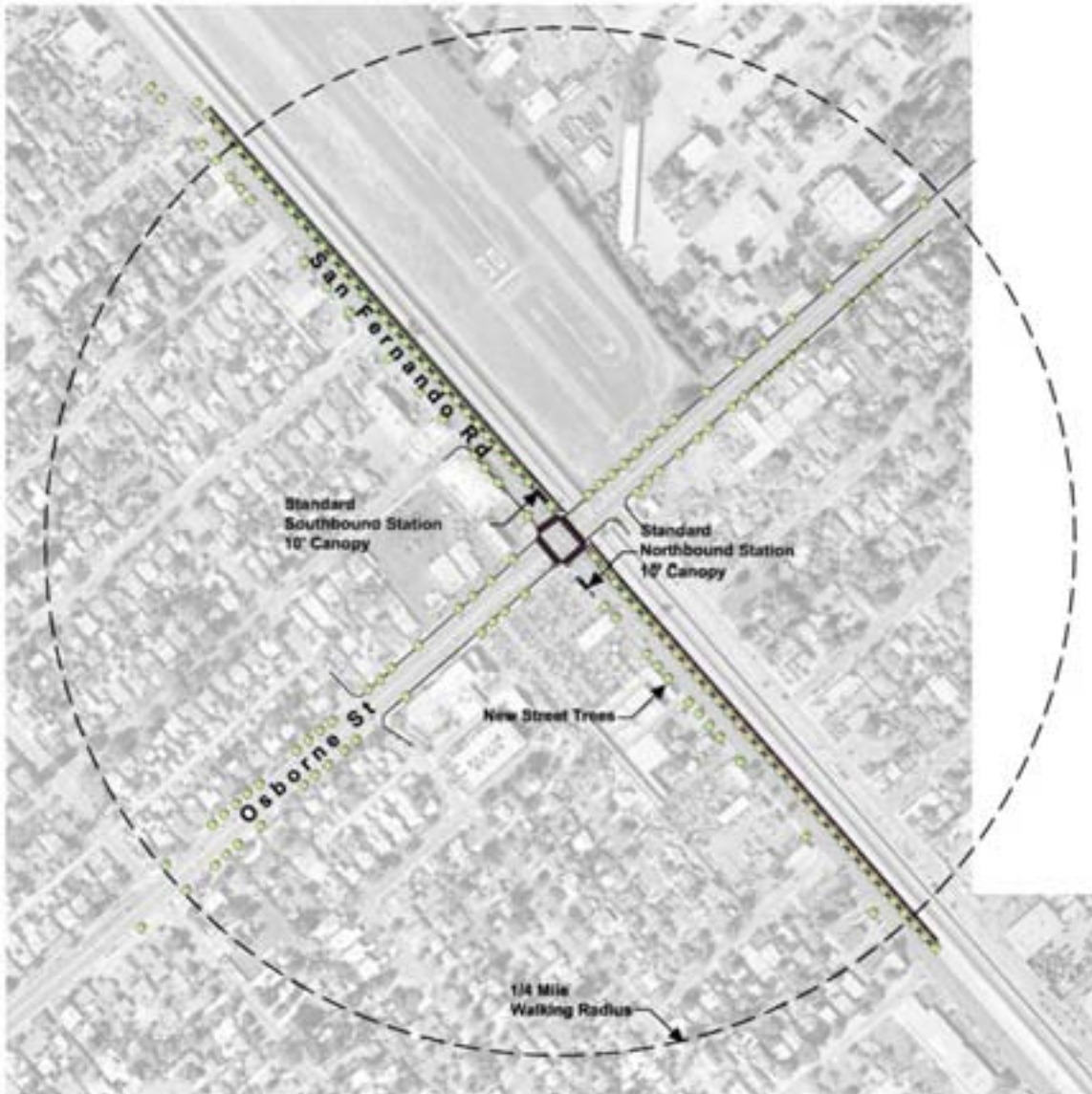
Figure 4-23. Typical Plan of Tree Planting Within ¼ Mile of Station (San Fernando / Osborne Station)
