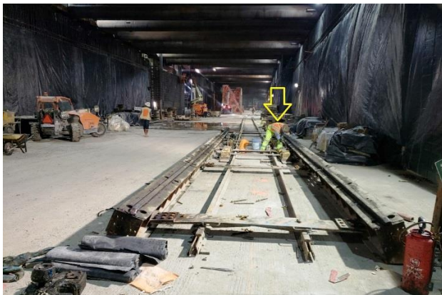
Temporary Rail Installation at Wilshire/Fairfax Station
