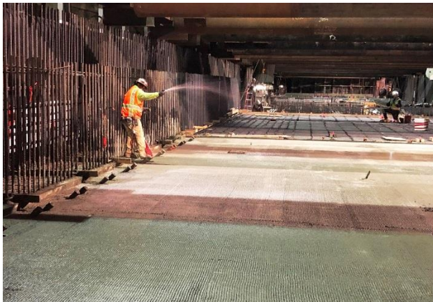
Invert Concrete Placement at Wilshire/La Cienega Station
