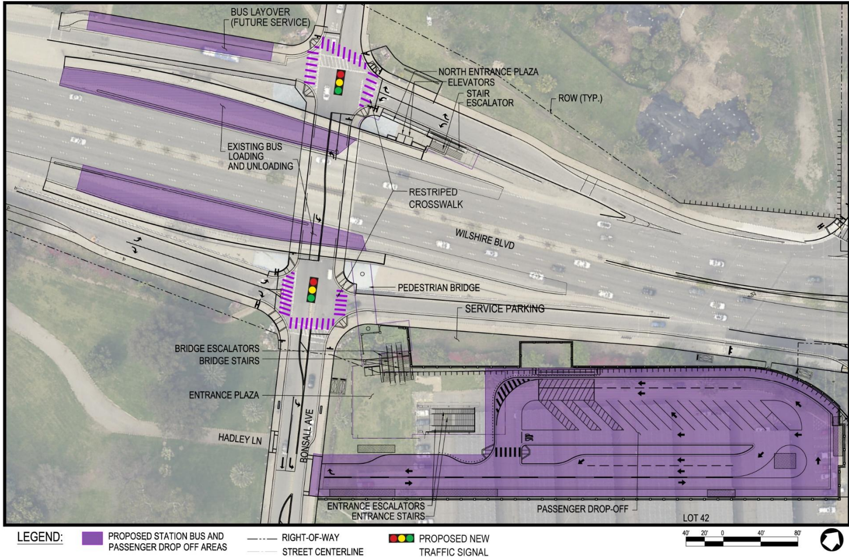
Figure 2-7: Bus and Passenger Drop-off Areas – Proposed
