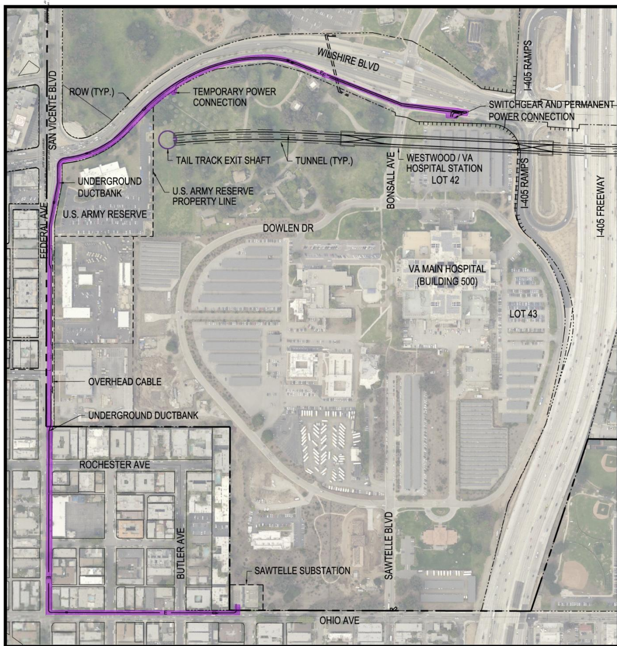
Figure 2-16: Temporary and Permanent Power
