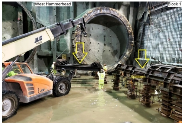
TBM Cradle Installation at Wilshire/Fairfax Station
