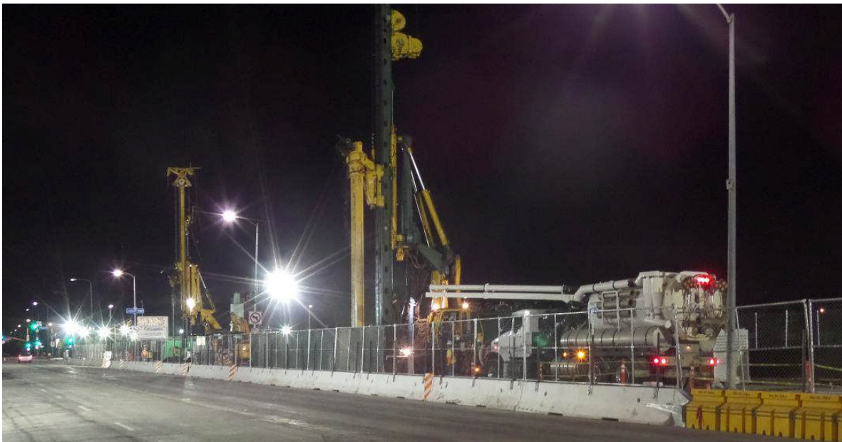
Drill Tec drilling Panel #24.
