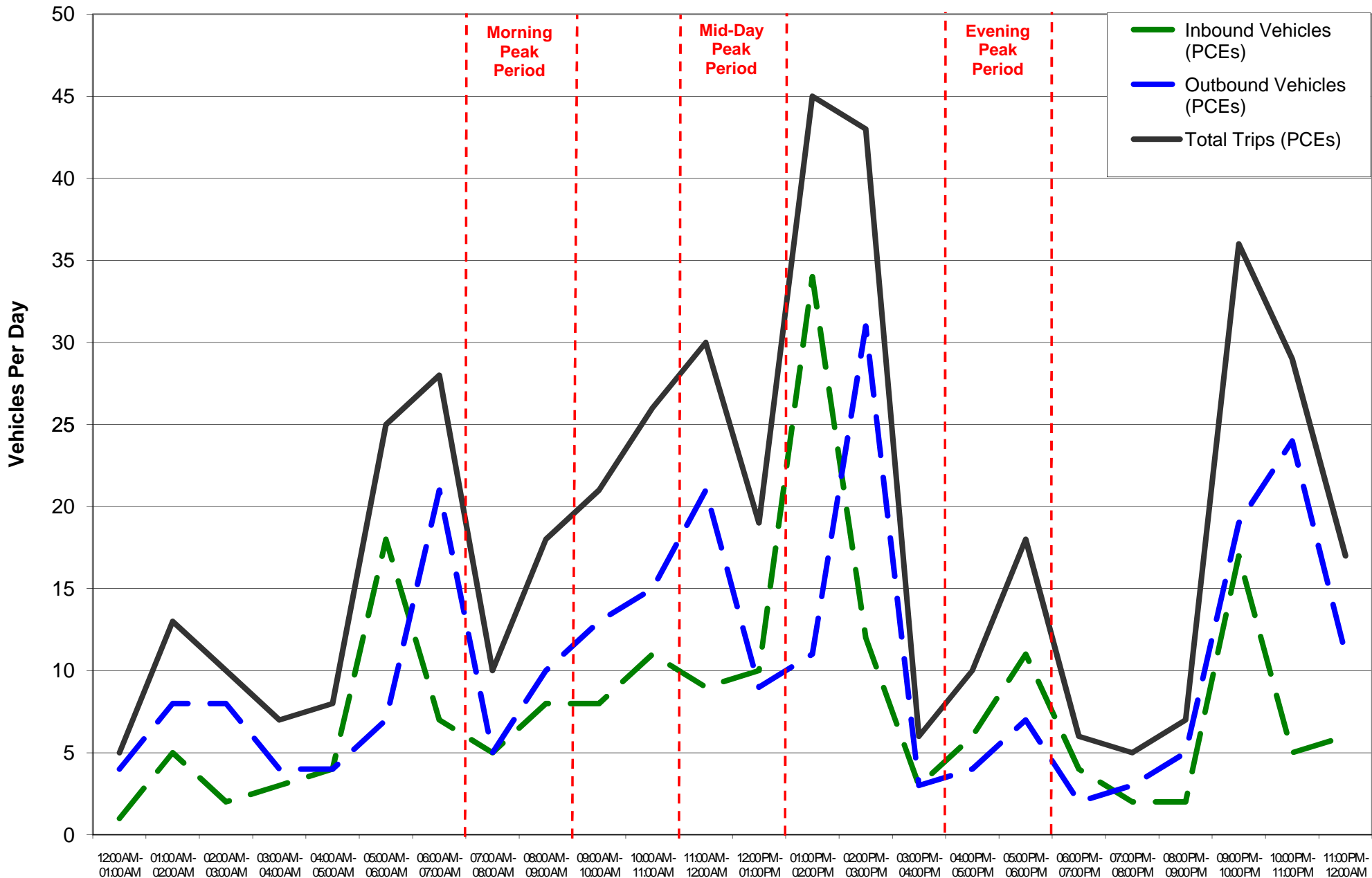
FIGURE 3 CRENSHAW/LAX TRANSIT CORRIDOR LRT MAINTAINANCE FACILITY TRIP GENERATION PROJECTION
