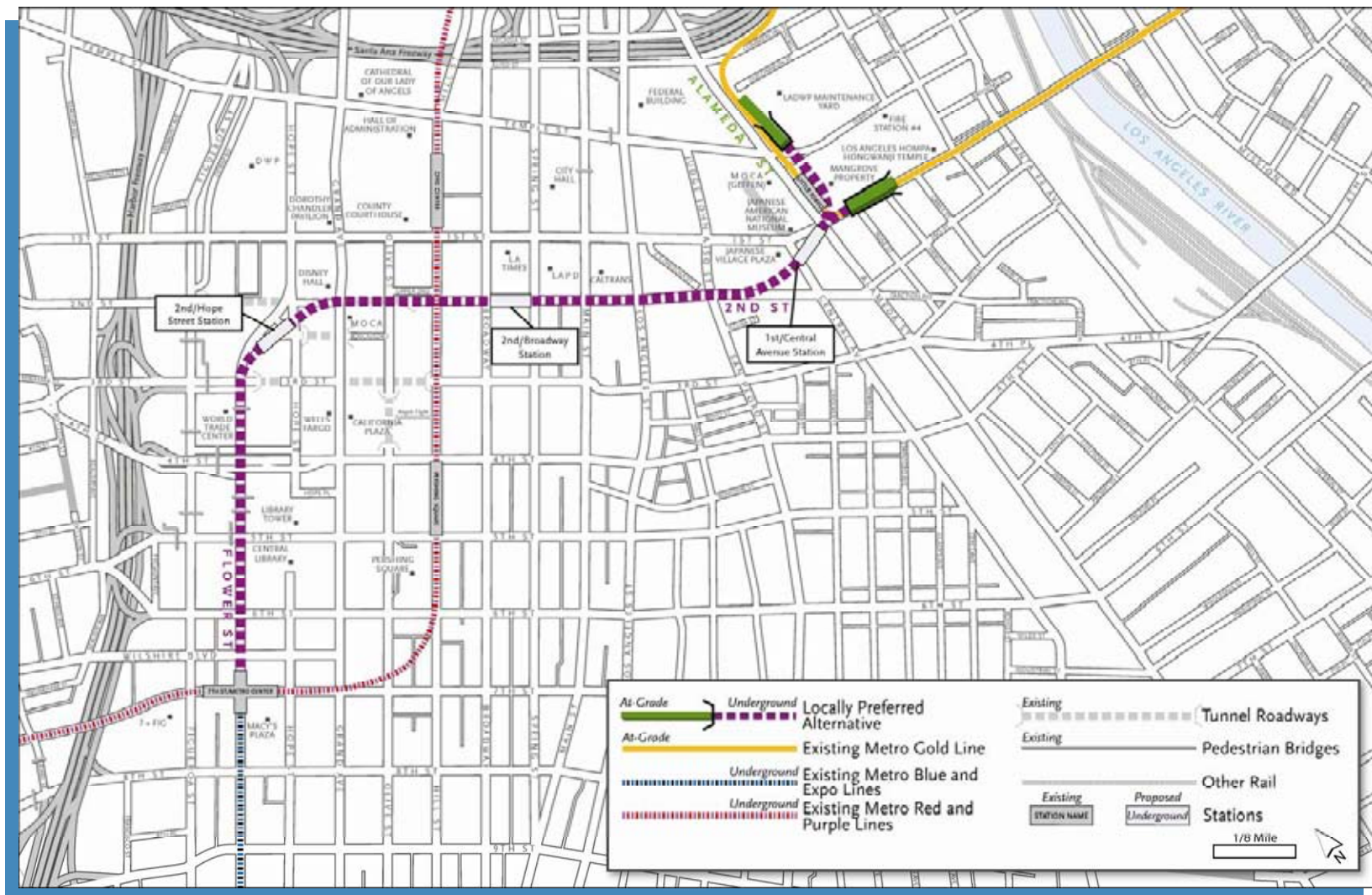
Figure 2-10. Locally Preferred Alternative
