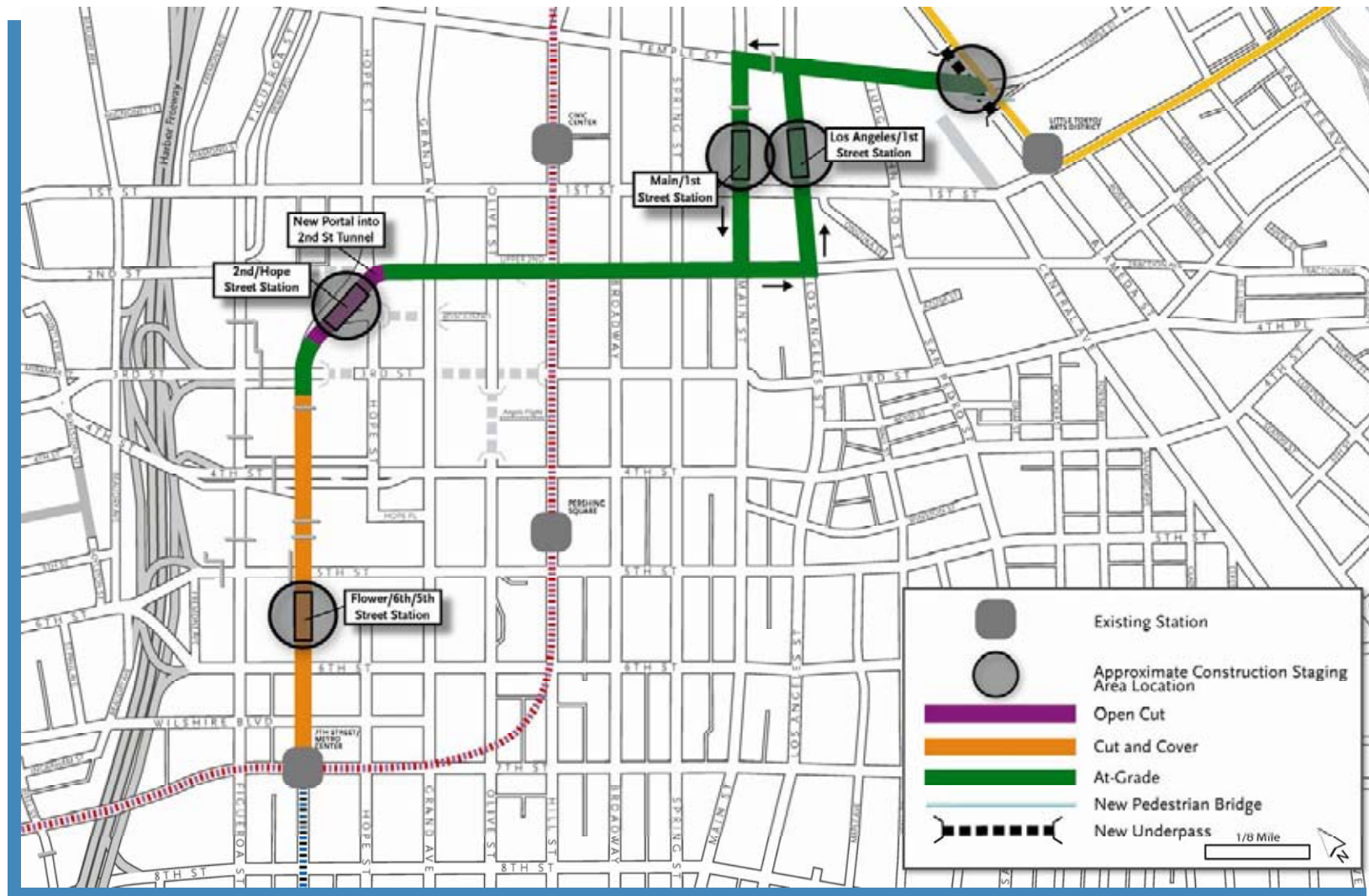
Figure 2-14. At-Grade Emphasis LRT Alternative Construction Areas and Methods
