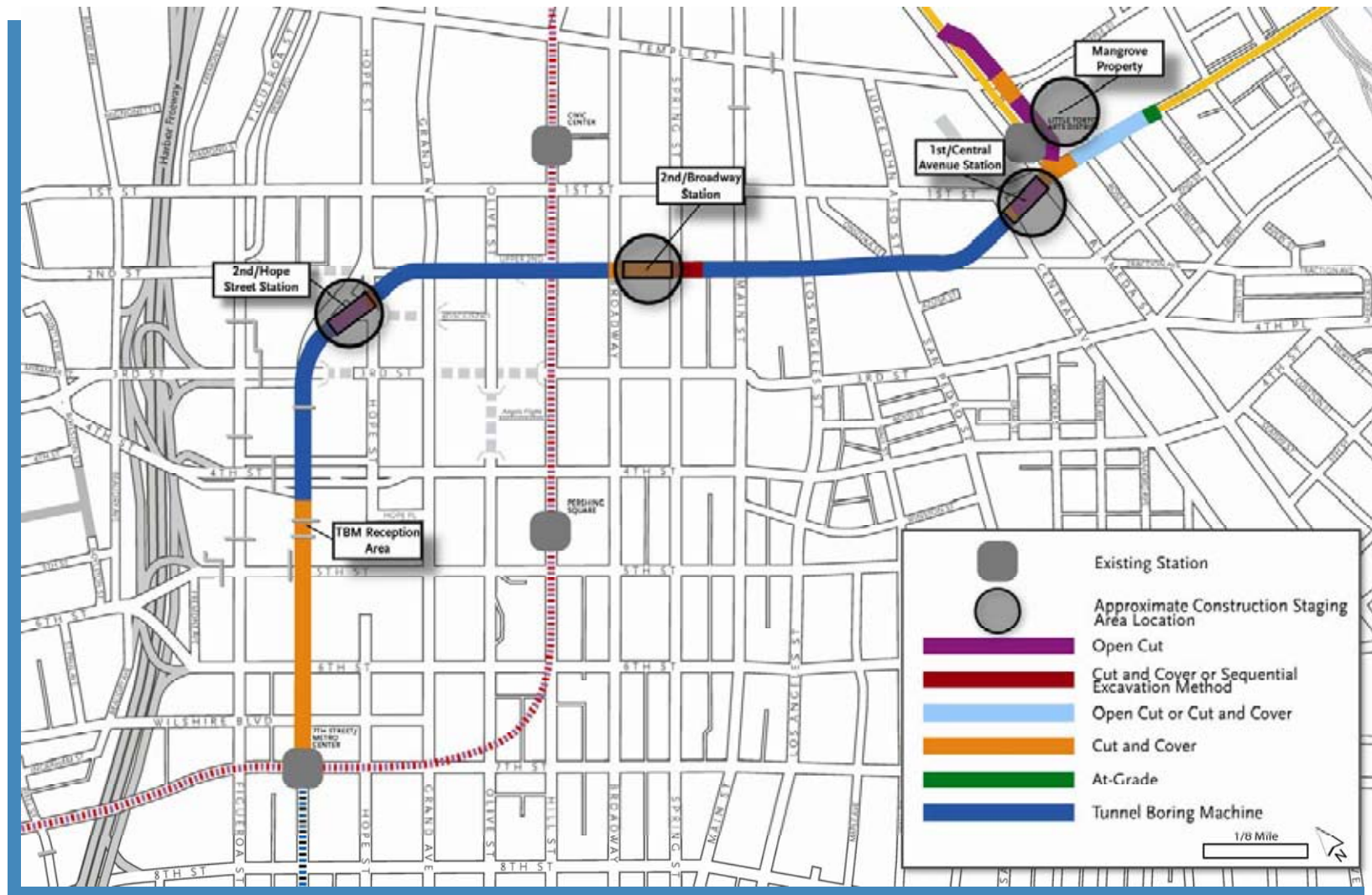
Figure 2-16. Locally Preferred Alternative Construction Areas and Methods
