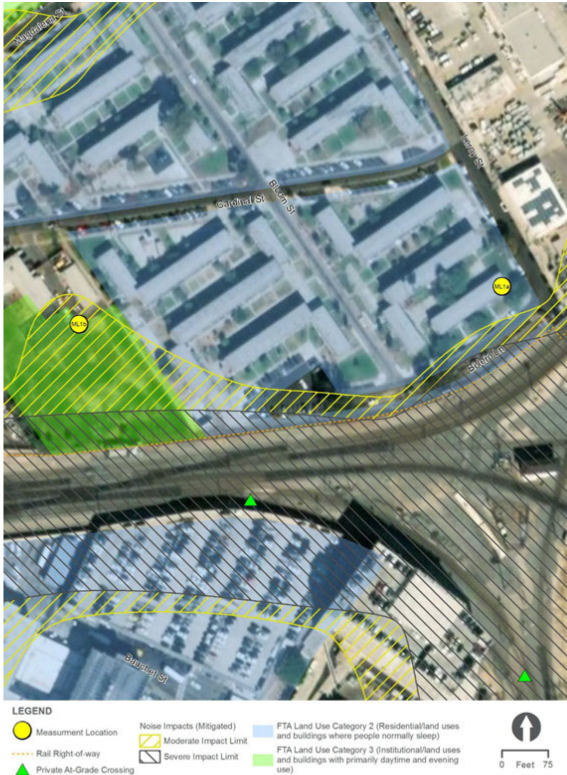
Figure 10-4. Noise Impact Areas at William Mead Homes – Proposed Project (2031 Condition with Mitigation)
