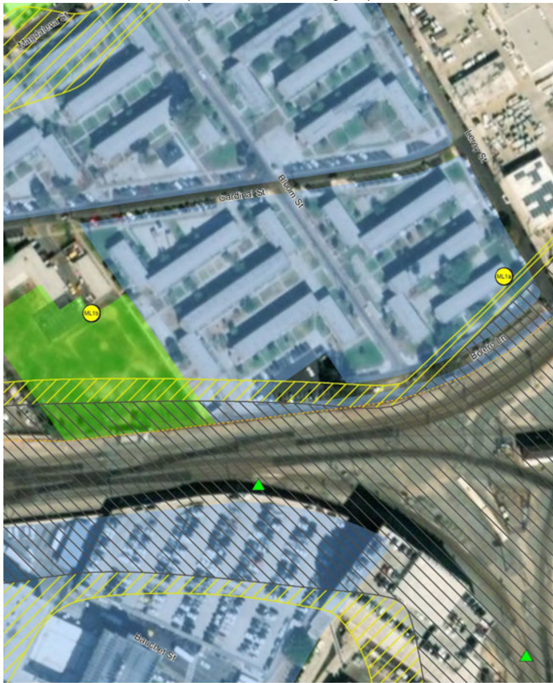
Figure 10-5. Noise Impact Areas at William Mead Homes – Build Alternative (2031 Condition with Mitigation)
