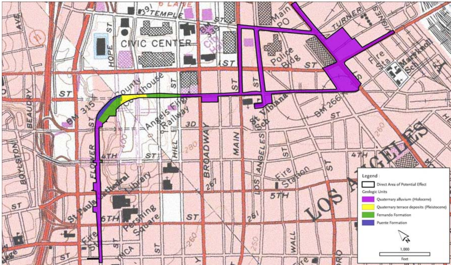
Figure 4-2. Geologic Map
