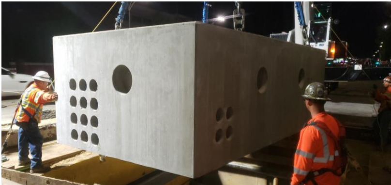
Vault installation along Van Nuys Bl between Vanowen St and Vose St
