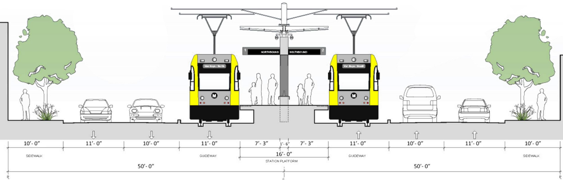
Concept Image. Typical ESFV street running section with station.
