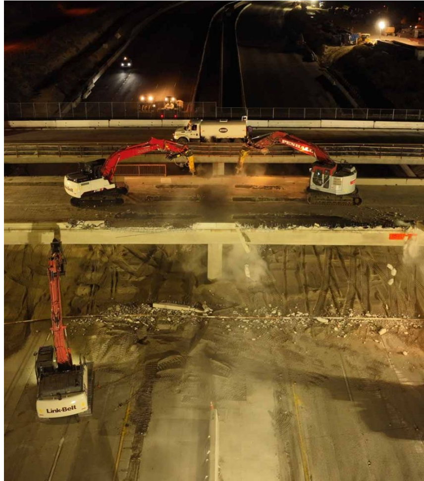
Stage 1 milestones – Weldon Canyon Rd Bridge demo, median construction, overhead sign removal
