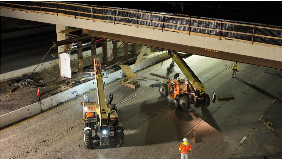
Weldon Canyon Overcrossing bridge falsework removal, May 2023
