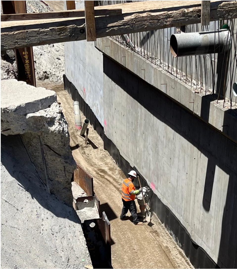
Backfilling of abutments at Weldon Canyon Rd Bridge, August 2023
