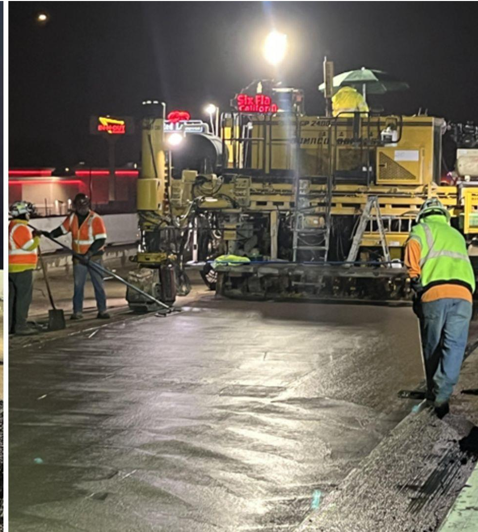
Concrete placement from Magic Mountain Pkwy to Valencia Bl, January 2024
