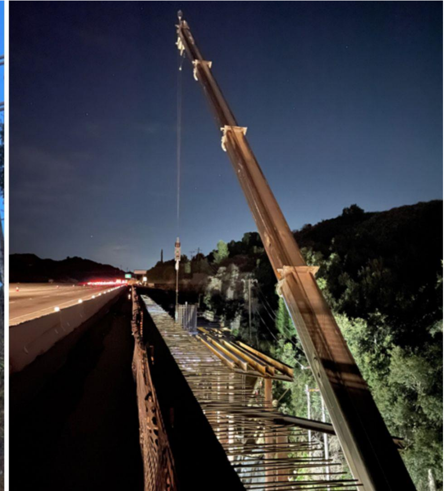
Falsework grading at Gavin Bridge, January 2024
